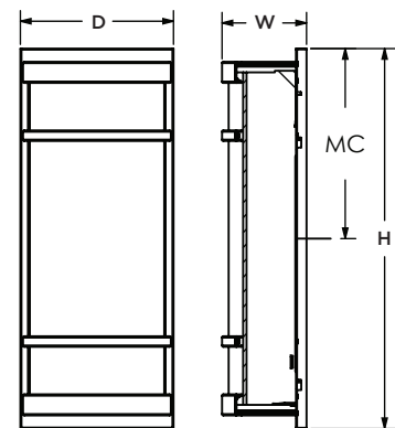
MC - Mounting Center
